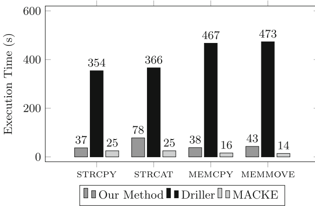
Fig. 4. Comparison of tools analysis time on the benchmark programs
