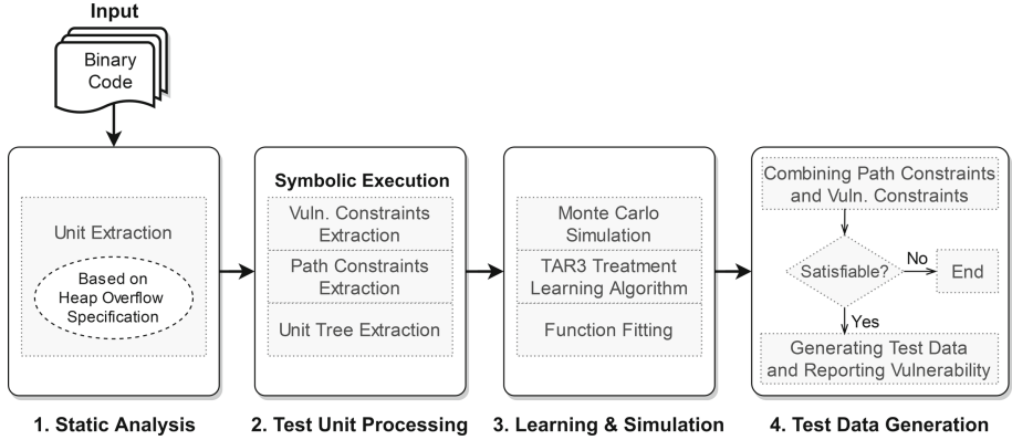
Fig. 1. Architecture of the proposed method
